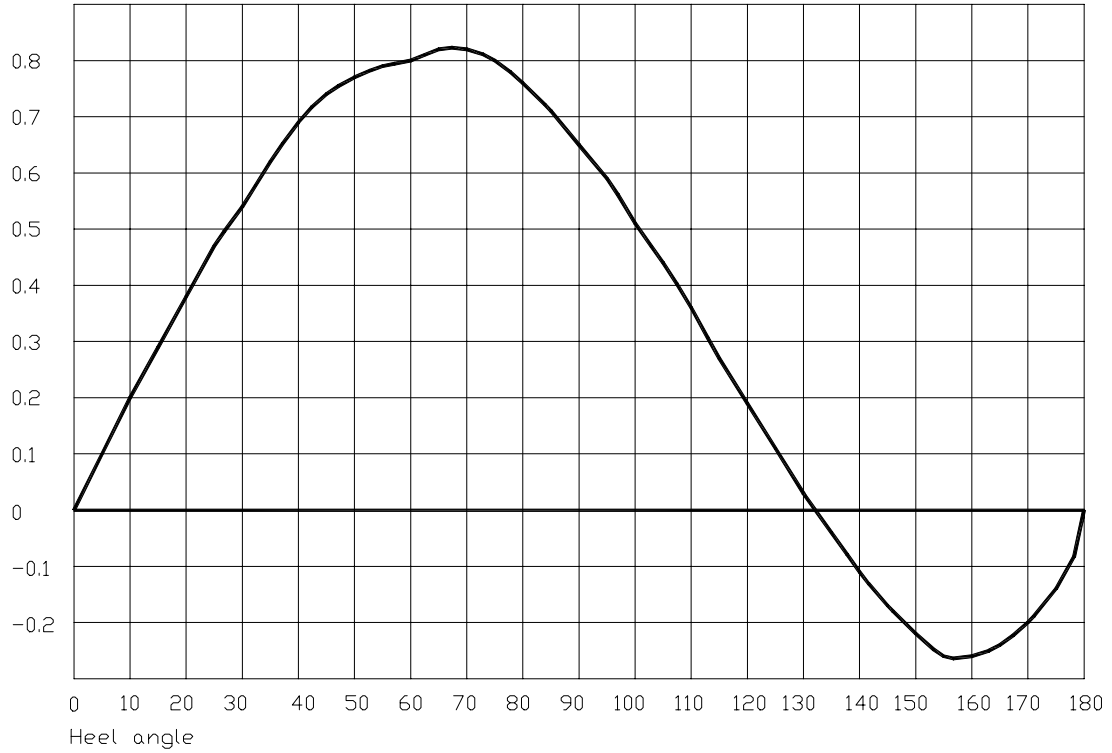
Stability curve for MALÖ 45 in min. sailing condition
