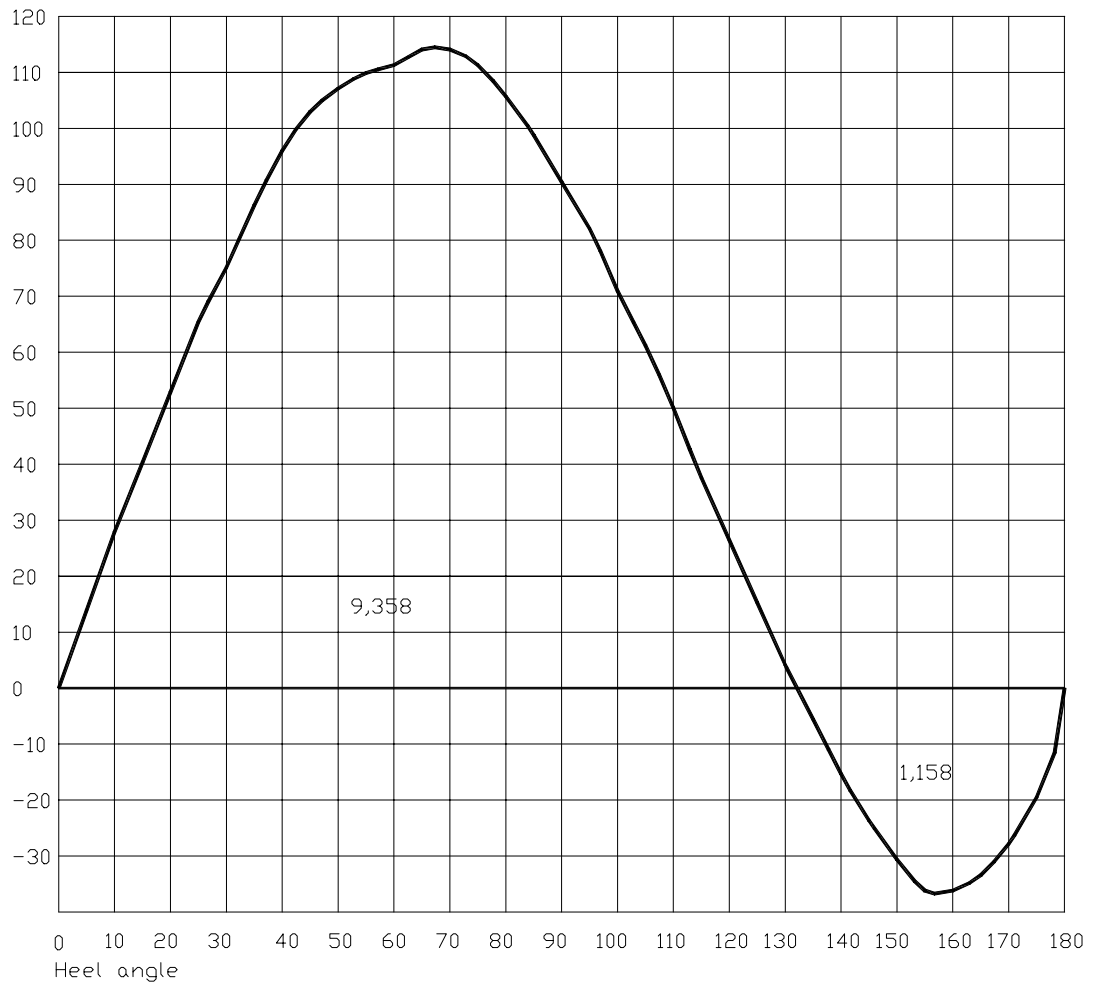
Stability curve for MALÖ 45 in min. sailing condition
