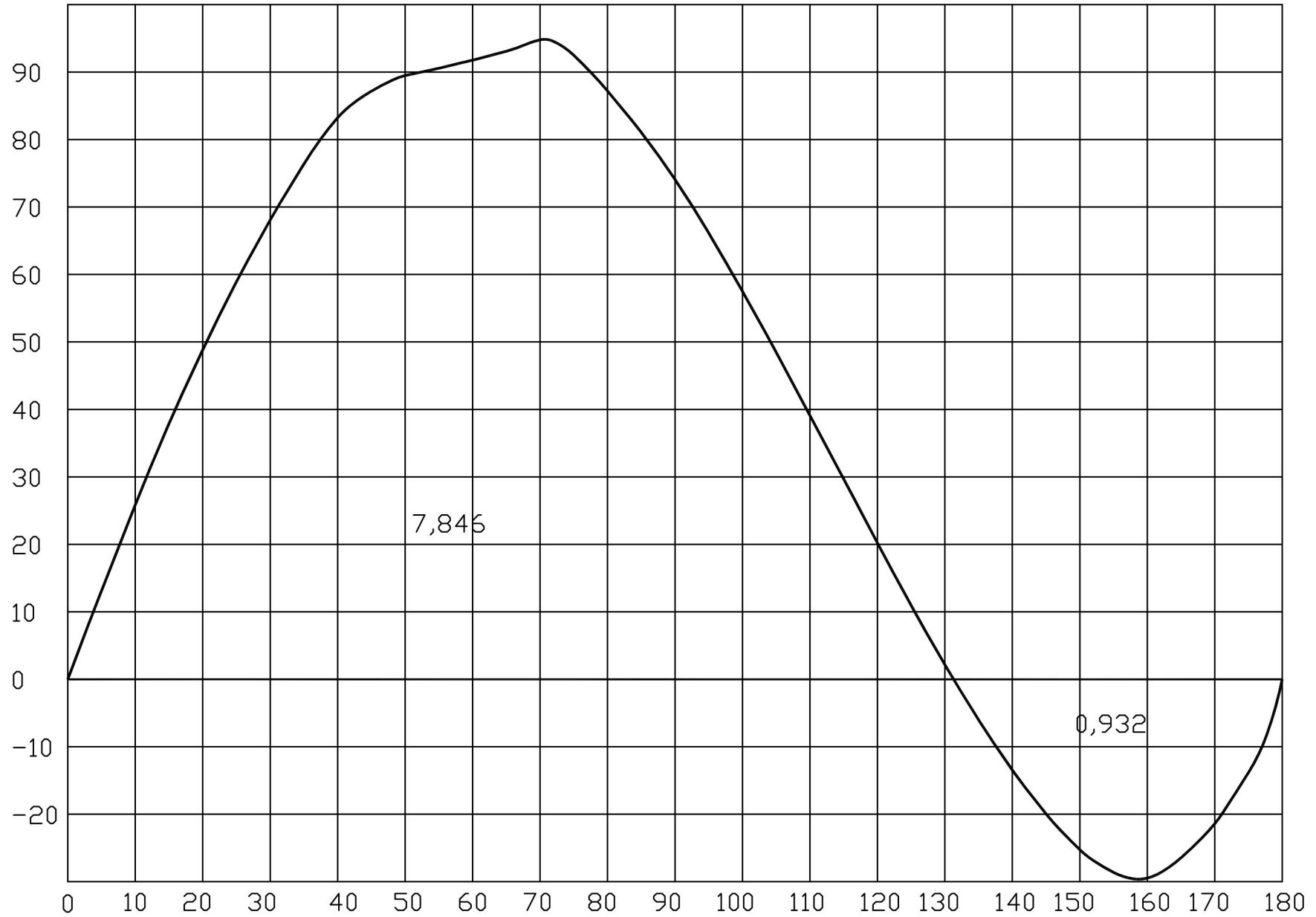
Stability curve for MALÖ 43 in min. sailing condition
